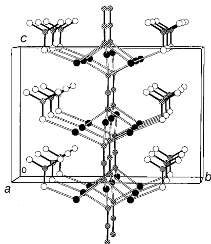
Figure 2. Crystal structure of \text{AgN}_3 \cdot 2\text{AgNO}_3 viewed along the a direction. The solid, cross-hatched and open circles represent Ag, N, and O atoms, respectively.
